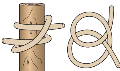
Securing to a piling using a clove hitch
